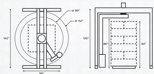
SONIC RTG
